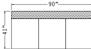
#53 3-CUSHION ARMLESS 90"
