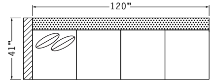
#84 LEFT ARM FACING/ RIGHT SIDE ARMLESS 120" + ARM
