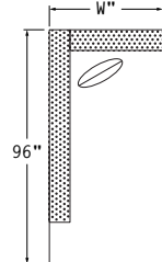
#99 LFBC LEFT FACING BUMPER CHAISE
