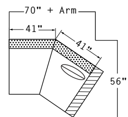
#79 RIGHT ARM FACING ANGLE 70" + ARM
