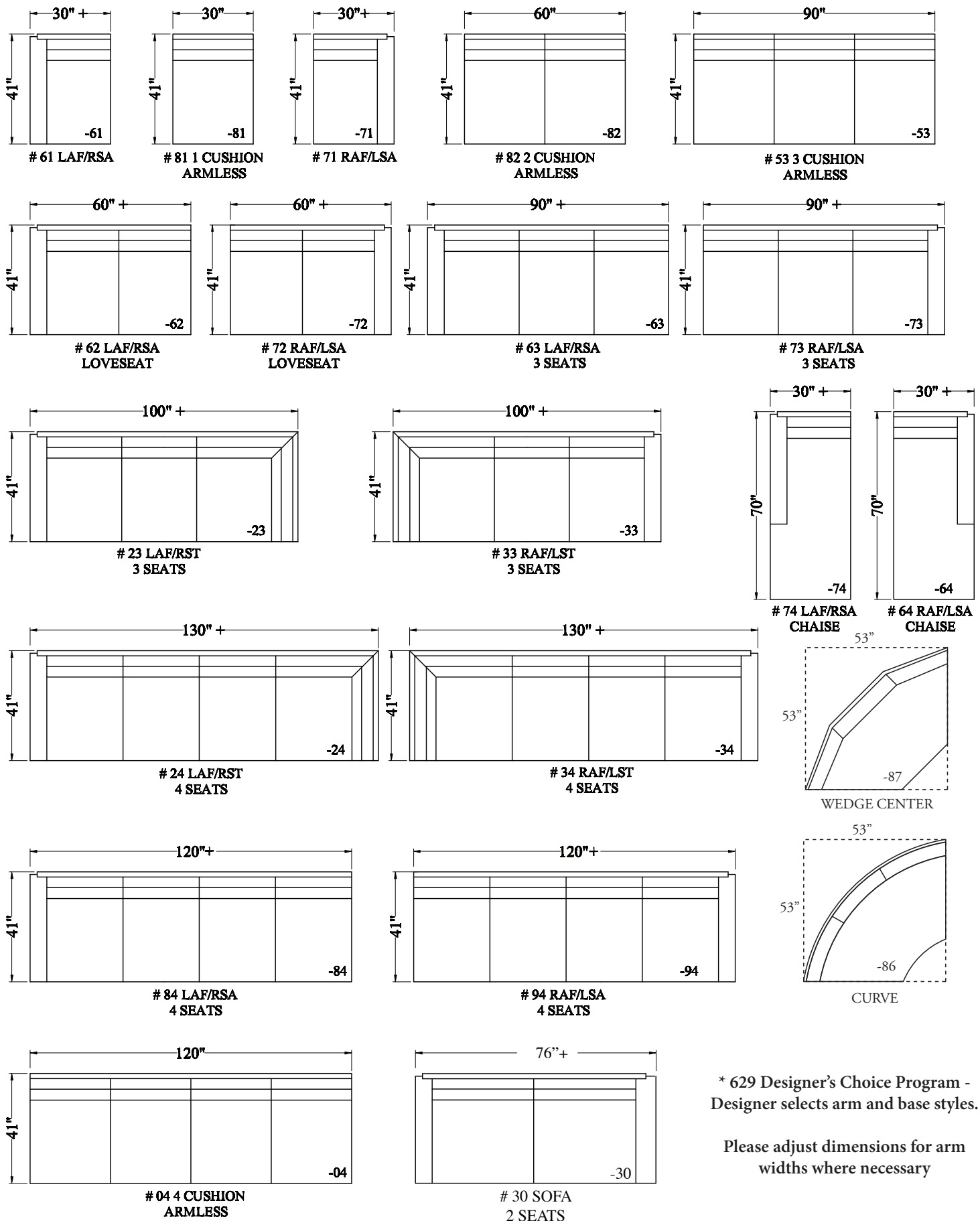
Schematic of 629 Designer's Choice - Sectional
